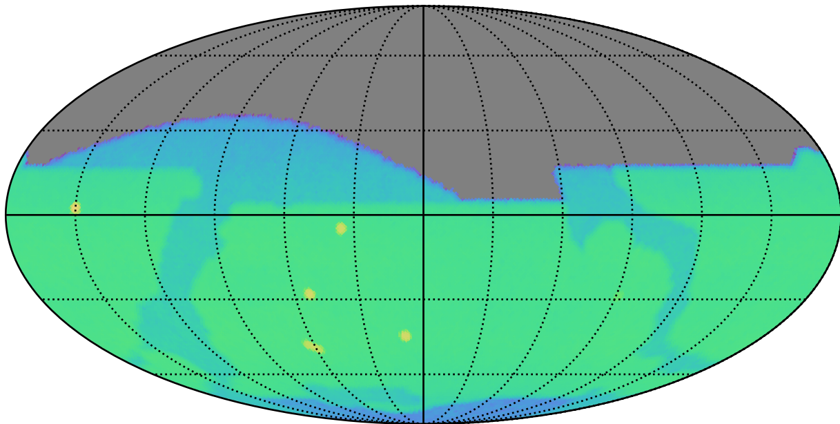
ddf_roll_deep_v3.5_10yrs z: CoaddM5
