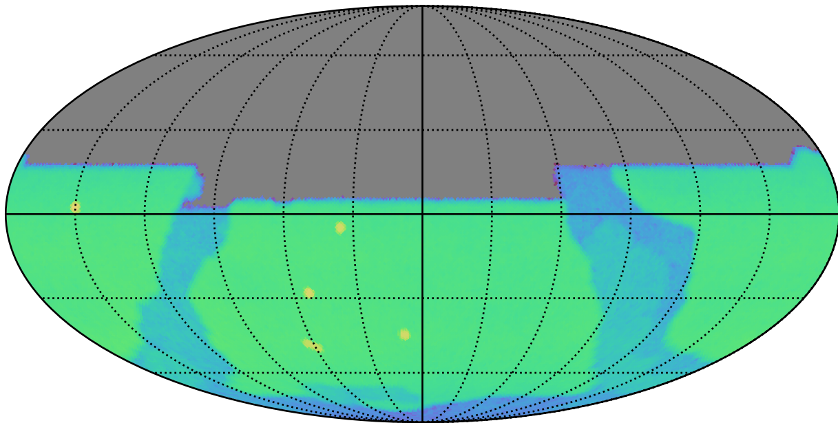
ddf_roll_deep_v3.5_10yrs y: CoaddM5
