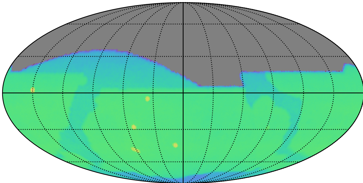
ddf_roll_deep_v3.5_10yrs r: CoaddM5
