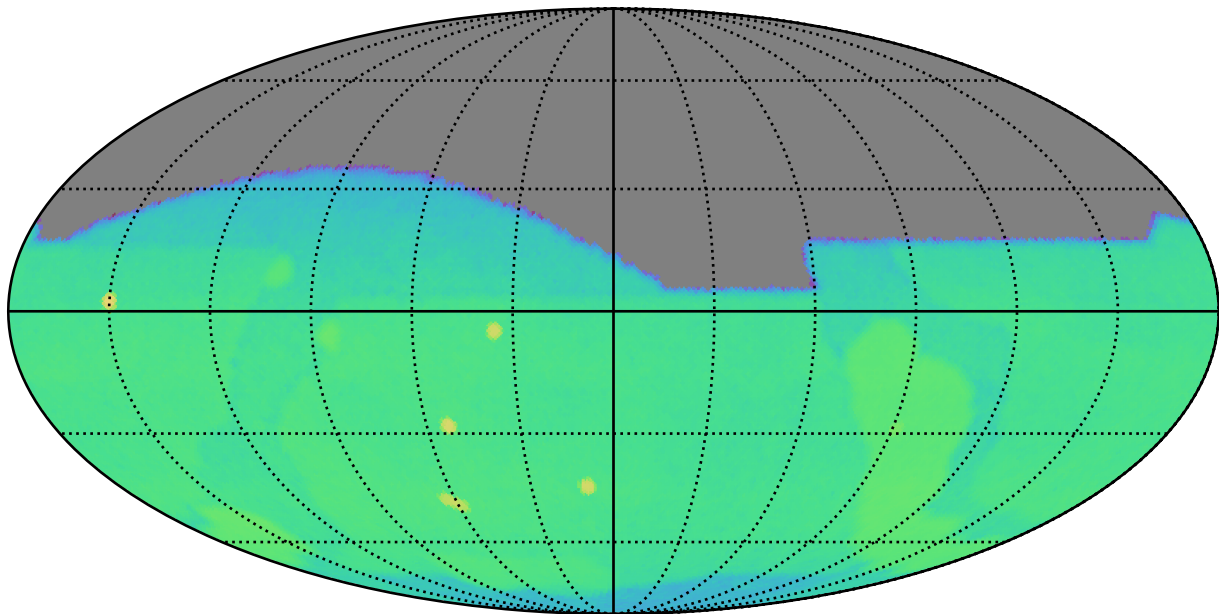
ddf_roll_deep_v3.5_10yrs g: CoaddM5
