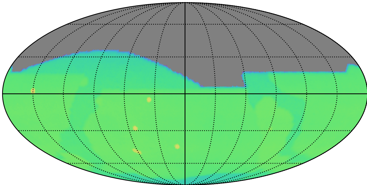
ddf_roll_deep_v3.5_10yrs : CoaddM5
