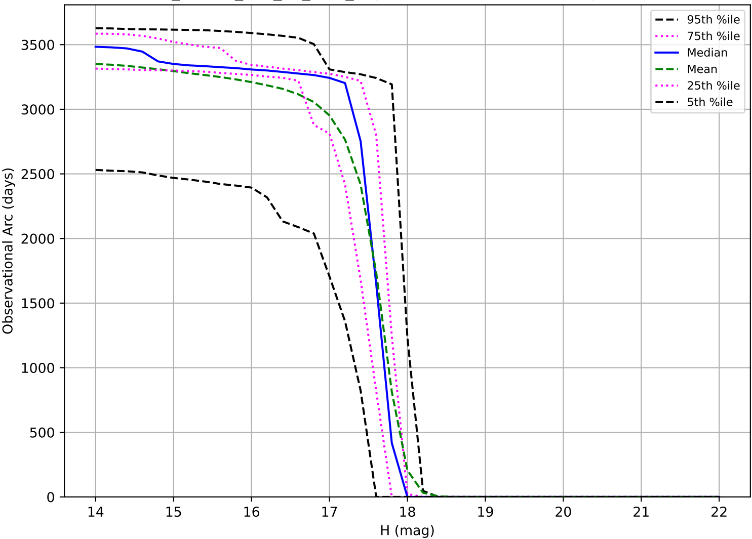
ddf_loaded_half_fl8_v3.4_10yrs: Observational Arc Length Trojan
