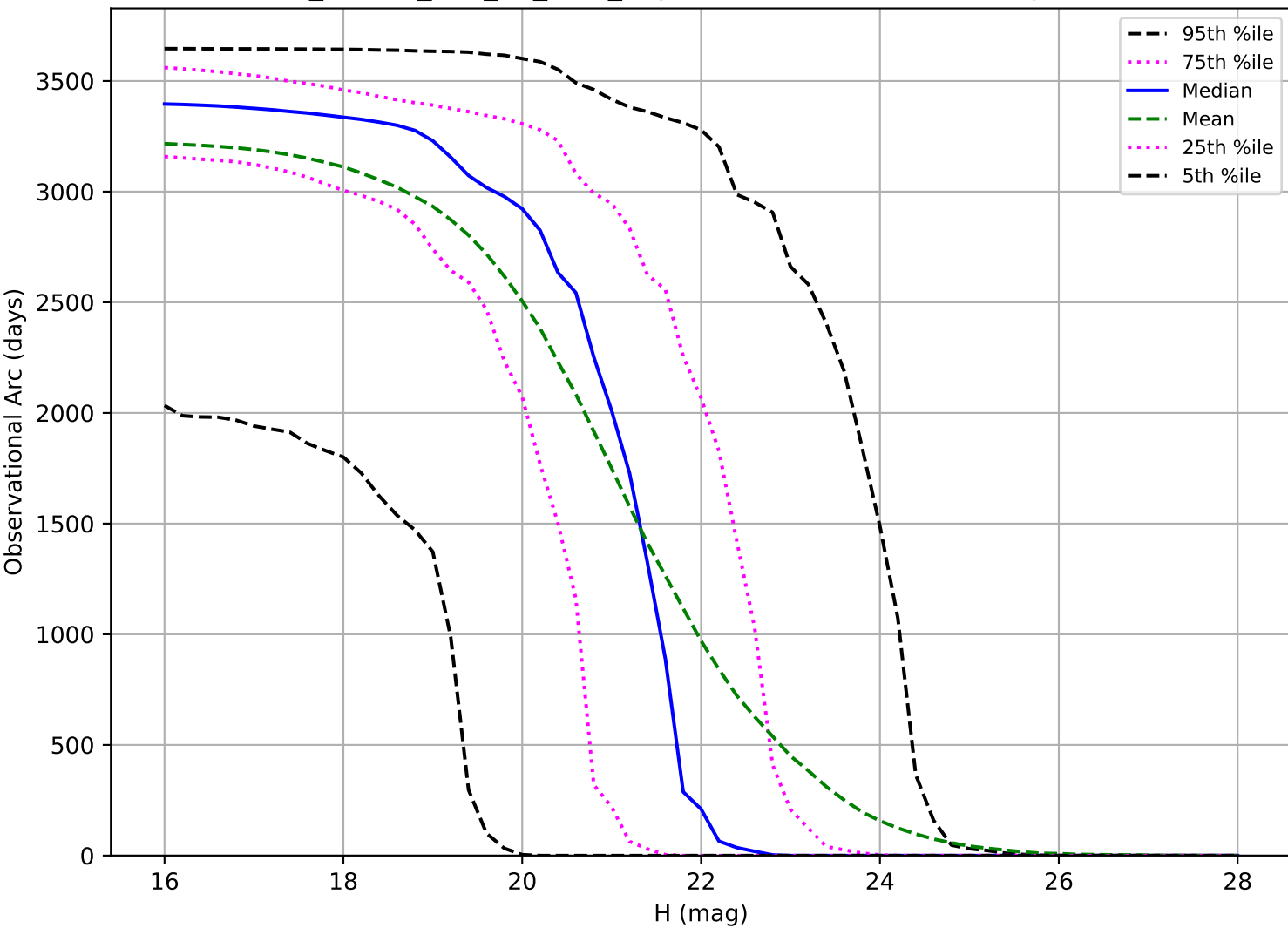
ddf_loaded_half_fl8_v3.4_10yrs: Observational Arc Length PHA
