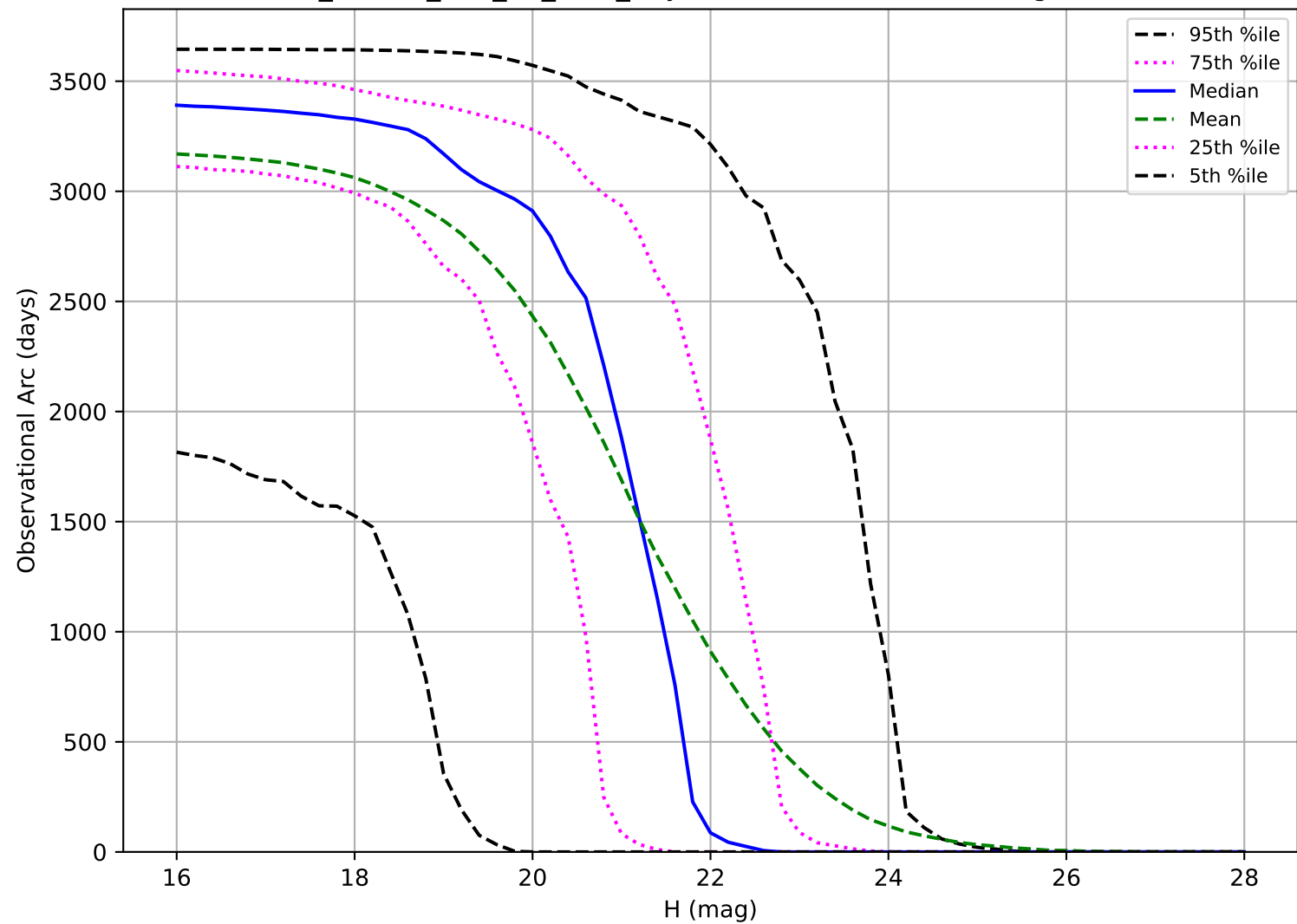
ddf_loaded_half_f18_v3.4_10yrs: Observational Arc Length NEO
