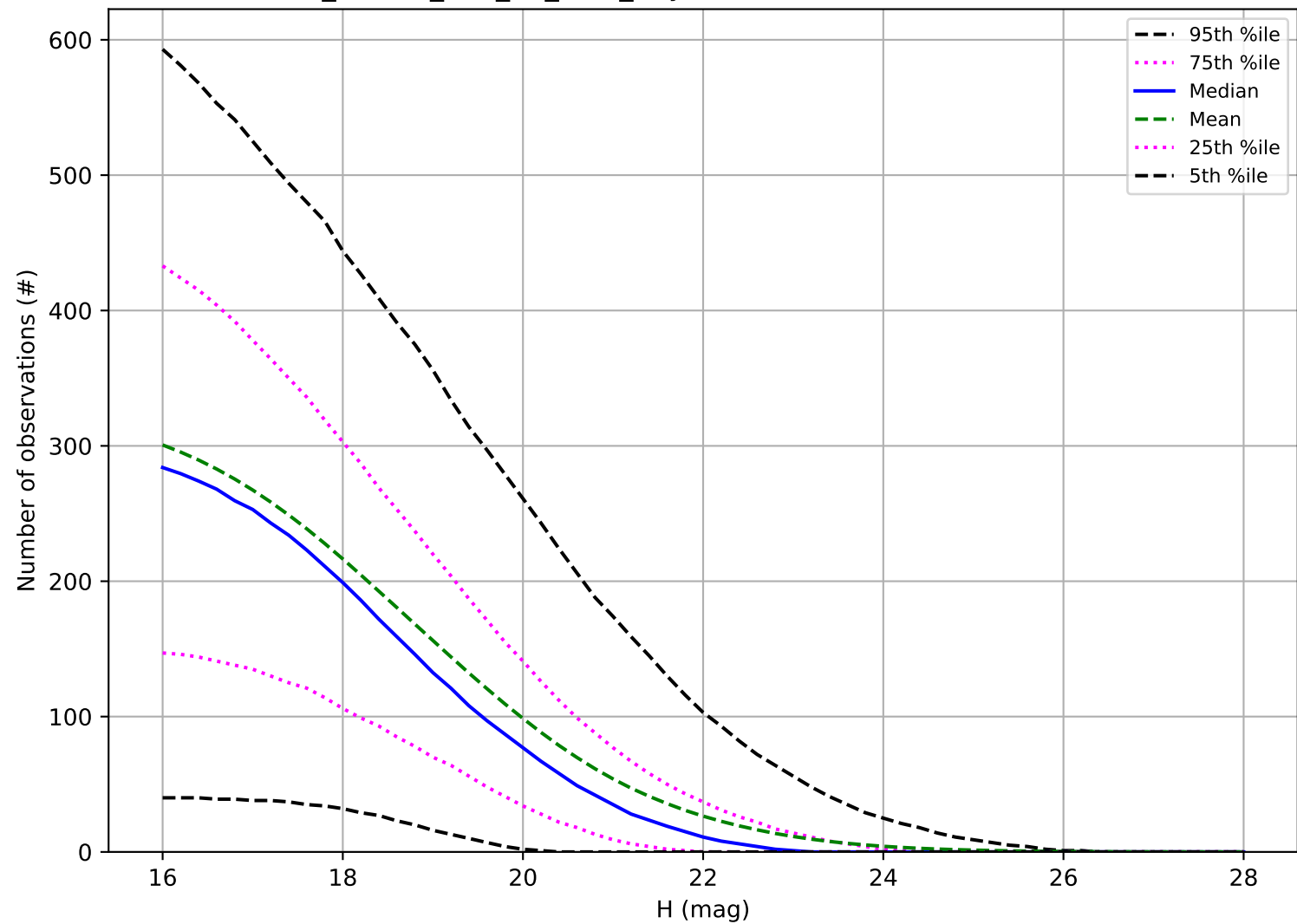
ddf_loaded_half_fl8_v3.4_10yrs: Number of observations PHA
