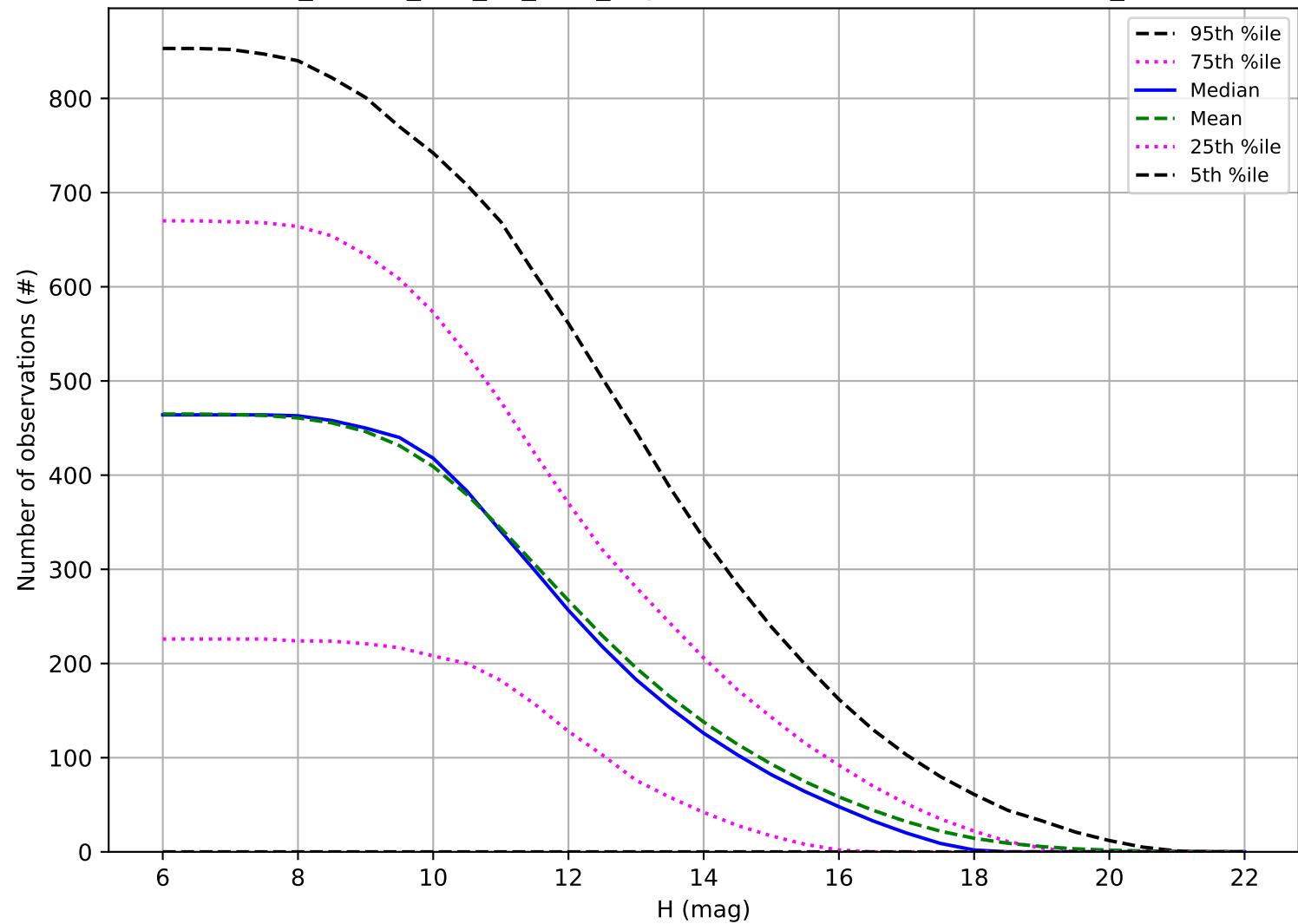
ddf_loaded_half_fl8_v3.4_10yrs: Number of observations OCC_r5
