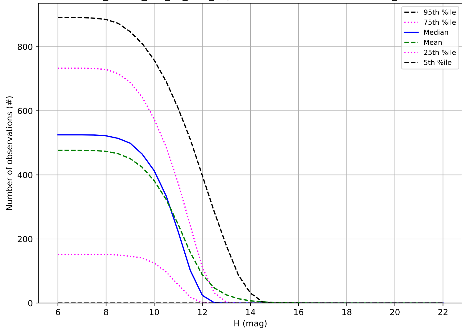
ddf_loaded_half_fl8_v3.4_10yrs: Number of observations OCC_r20
