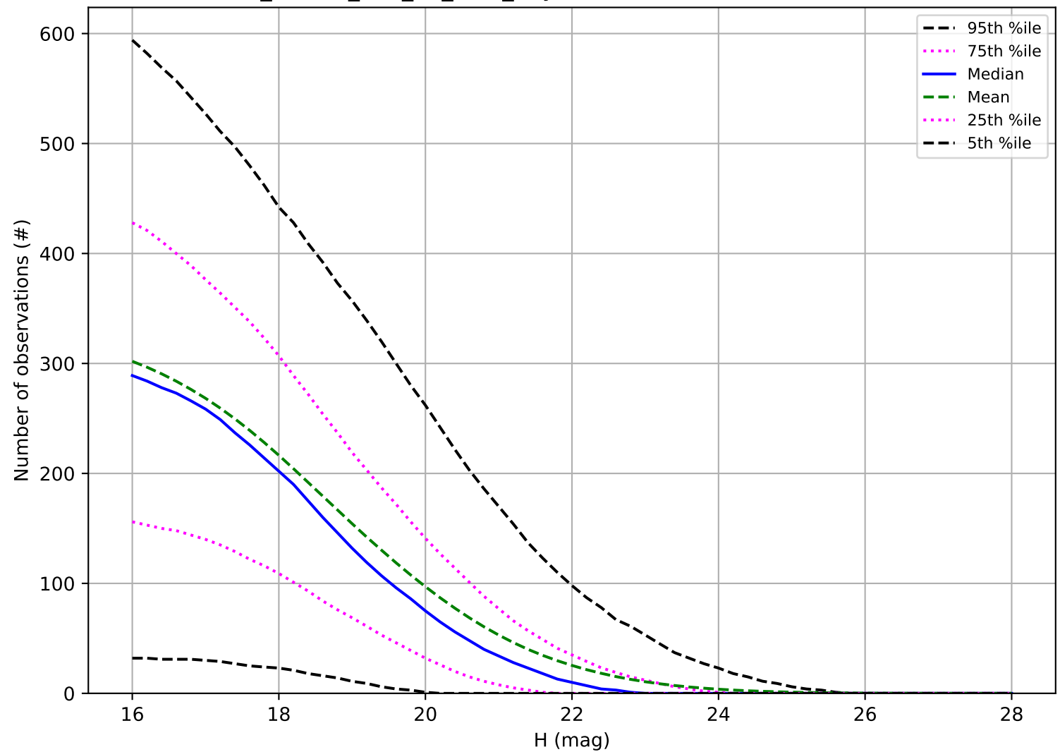
ddf_loaded_half_f18_v3.4_10yrs: Number of observations NEO
