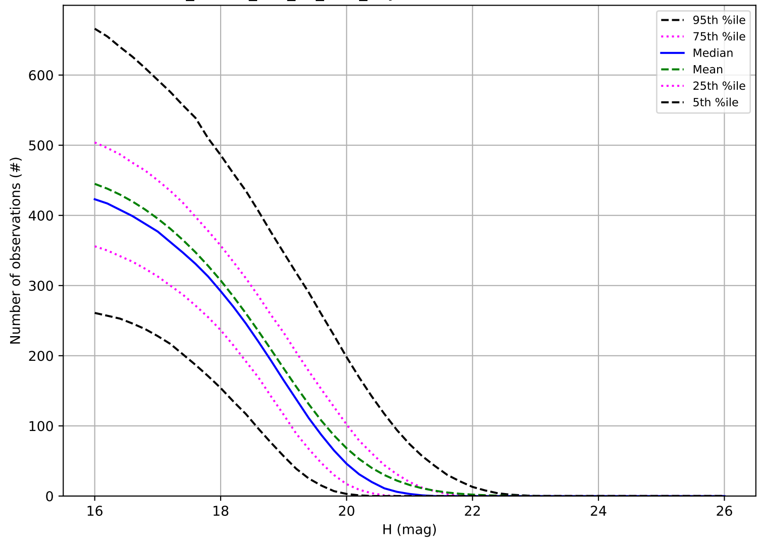
ddf_loaded_half_f18_v3.4_10yrs: Number of observations MBA
