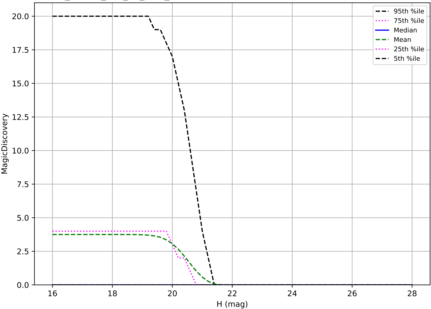
ddf_loaded_half_fl8_v3.4_10yrs: Vatira 6 detections in 60 nights detection loss
