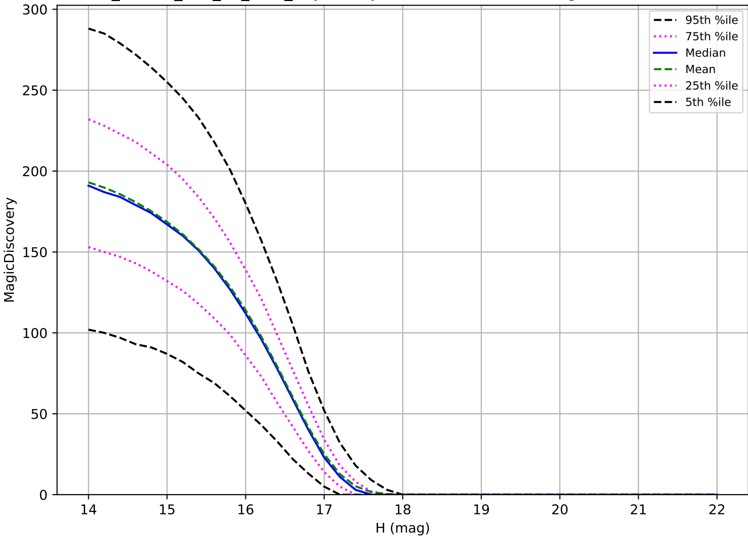
ddf_loaded_half_fl8_v3.4_10yrs: Trojan 6 detections in 60 nights detection loss
