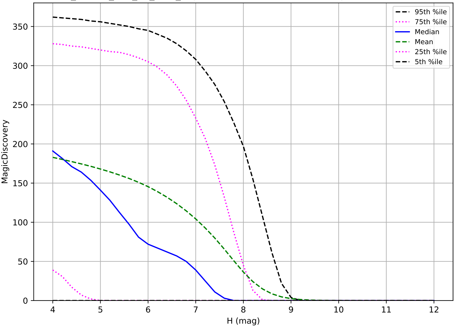
ddf_loaded_half_f18_v3.4_10yrs: TNO 6 detections in 60 nights detection loss
