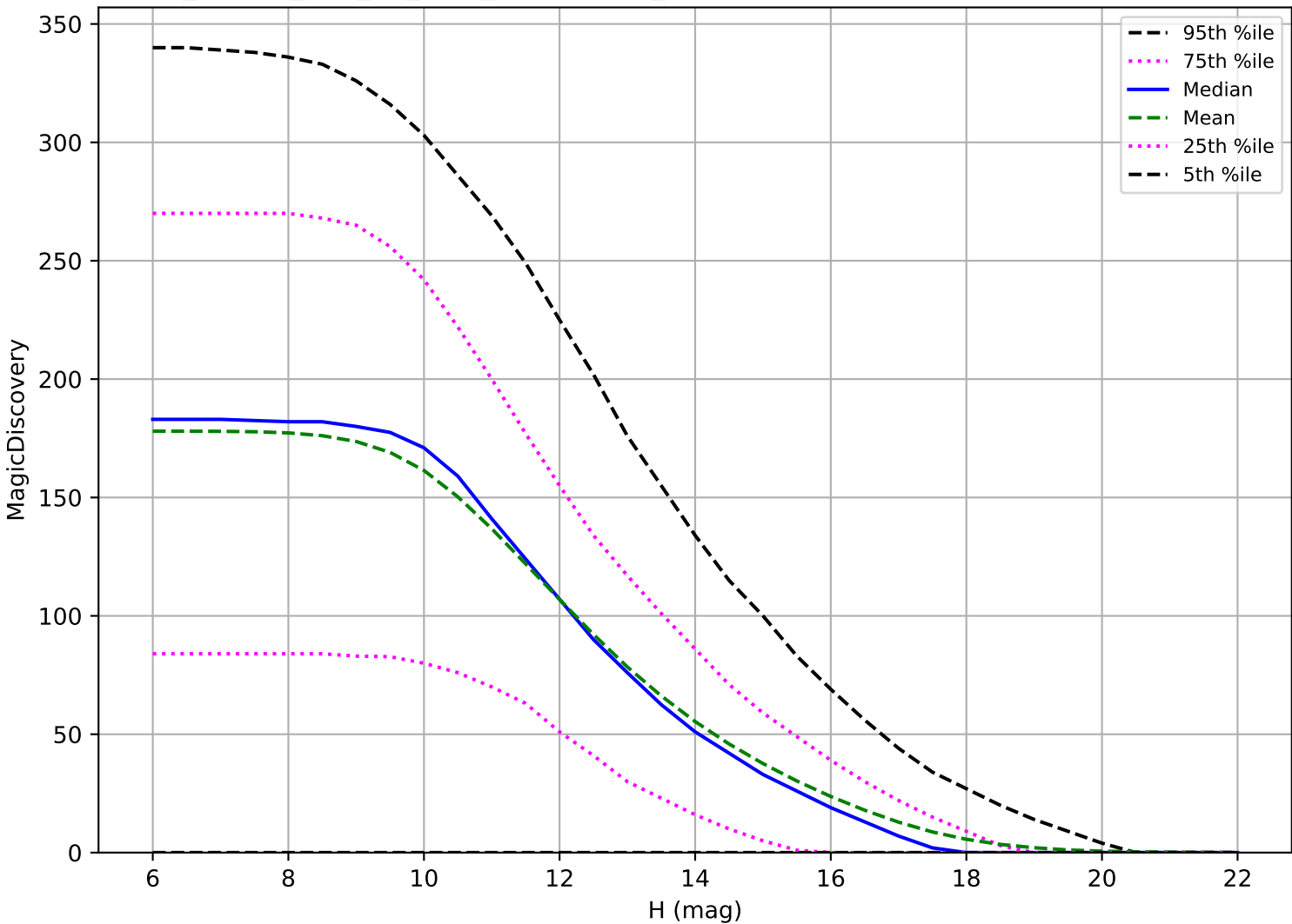
ddf_loaded_half_fl8_v3.4_10yrs: OCC_r5 6 detections in 60 nights detection loss
