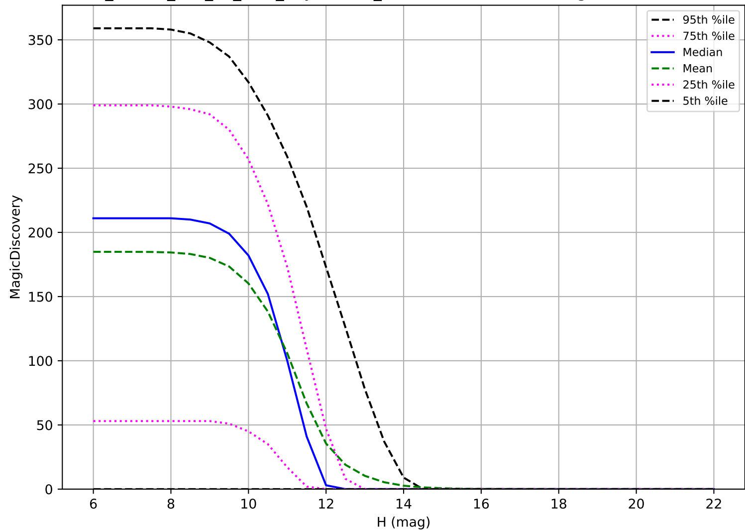
ddf_loaded_half_f18_v3.4_10yrs: OCC_r20 6 detections in 60 nights detection loss
