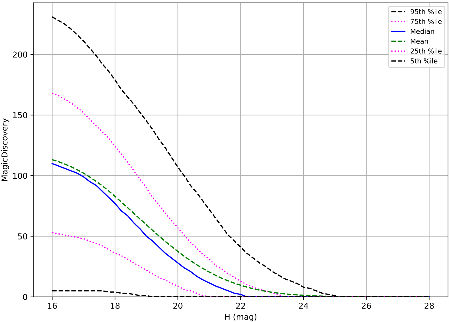
ddf_loaded_half_fl8_v3.4_10yrs: NEO 6 detections in 60 nights detection loss
