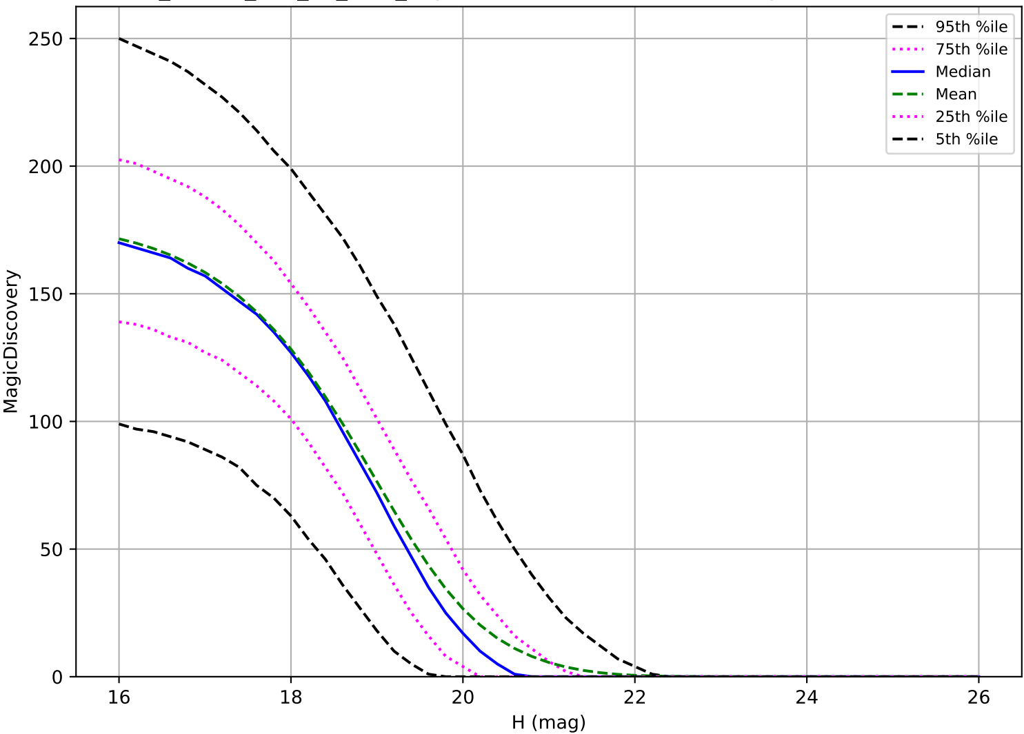
ddf_loaded_half_fl8_v3.4_10yrs: MBA 6 detections in 60 nights detection loss
