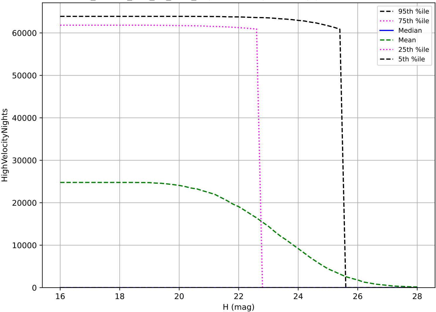
ddf_loaded_half_fl8_v3.4_10yrs: PHA High velocity pair detection loss
