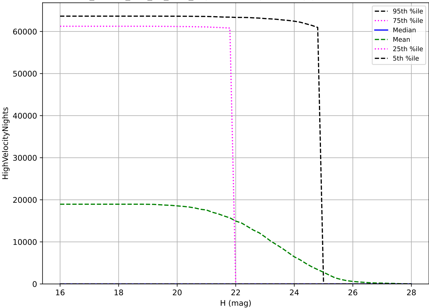
ddf_loaded_half_fl8_v3.4_10yrs: NEO High velocity pair detection loss
