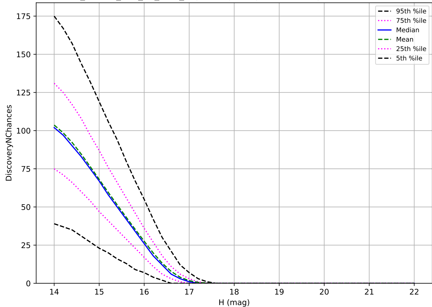
ddf_loaded_half_fl8_v3.4_10yrs: Trojan 3 pairs in 15 nights detection loss
