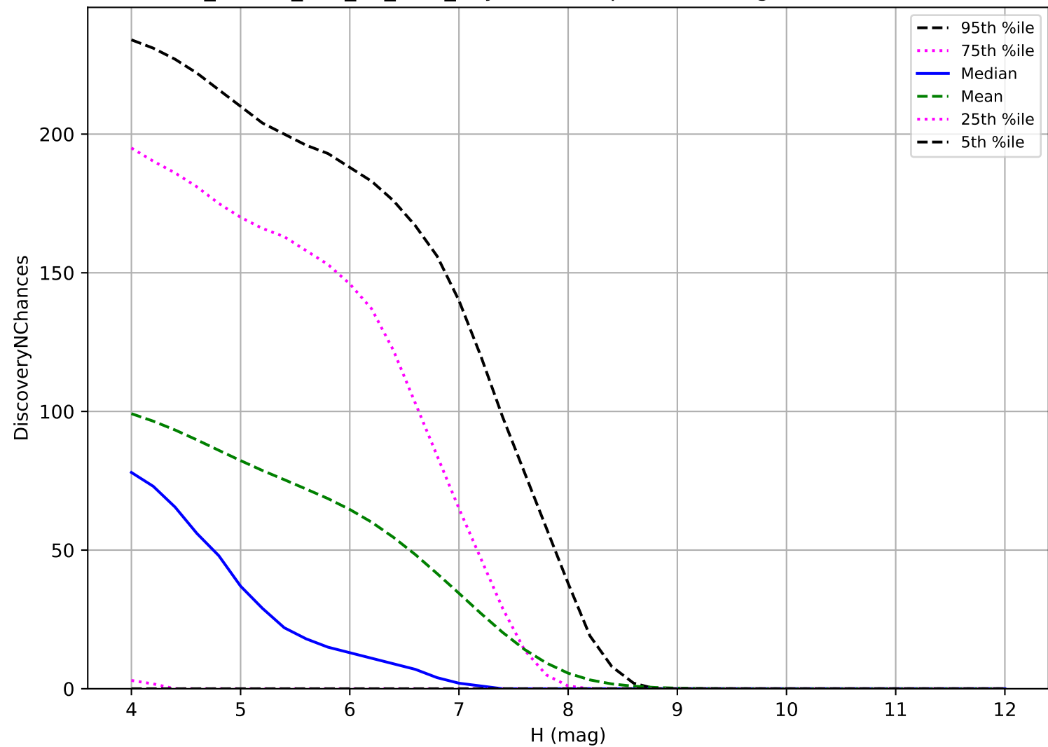
ddf_loaded_half_fl8_v3.4_10yrs: TNO 3 pairs in 15 nights detection loss
