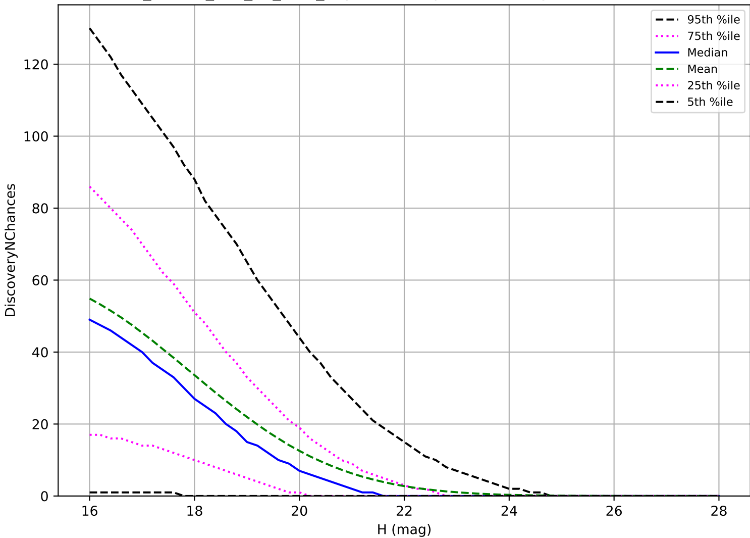
ddf_loaded_half_fl8_v3.4_10yrs: PHA 3 pairs in 15 nights detection loss
