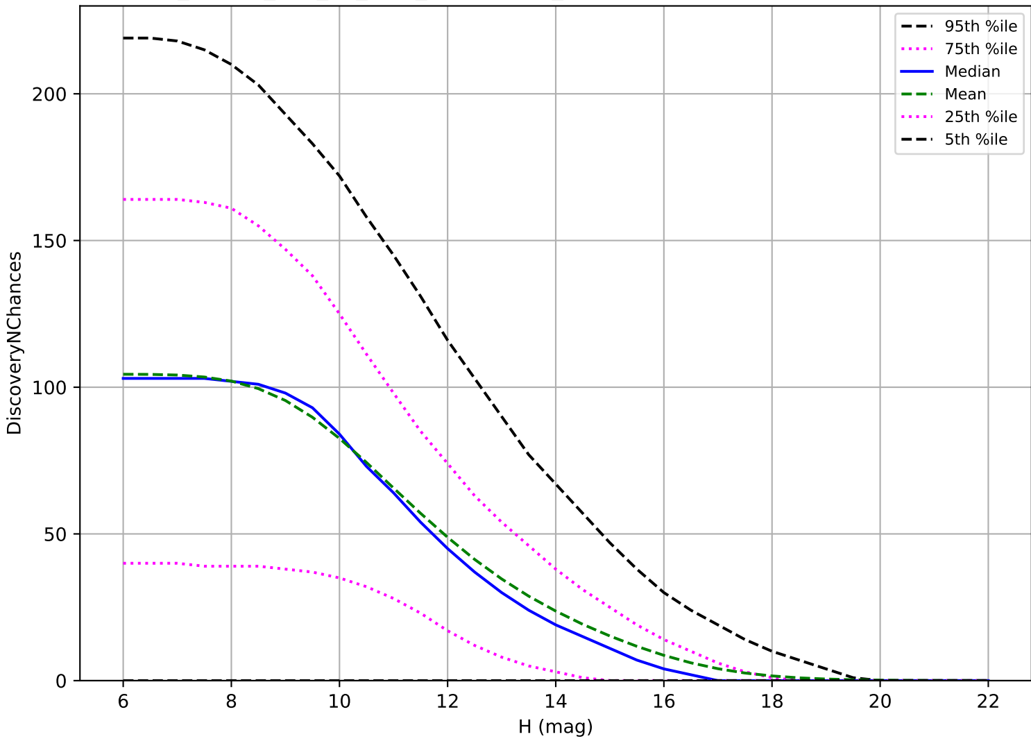
ddf_loaded_half_fl8_v3.4_10yrs: OCC_r5 3 pairs in 15 nights detection loss
