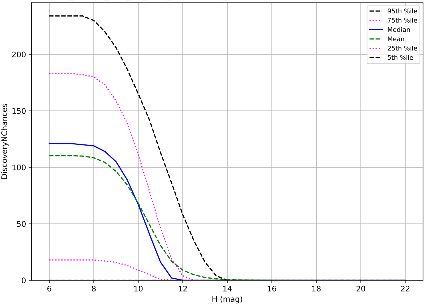
ddf_loaded_half_f18_v3.4_10yrs: OCC_r20 3 pairs in 15 nights detection loss
