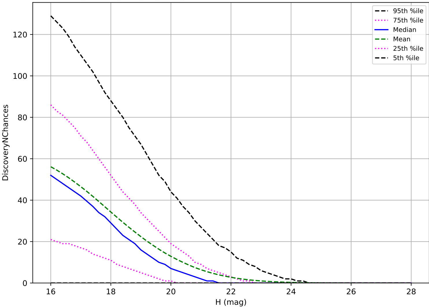
ddf_loaded_half_fl8_v3.4_10yrs: NEO 3 pairs in 15 nights detection loss
