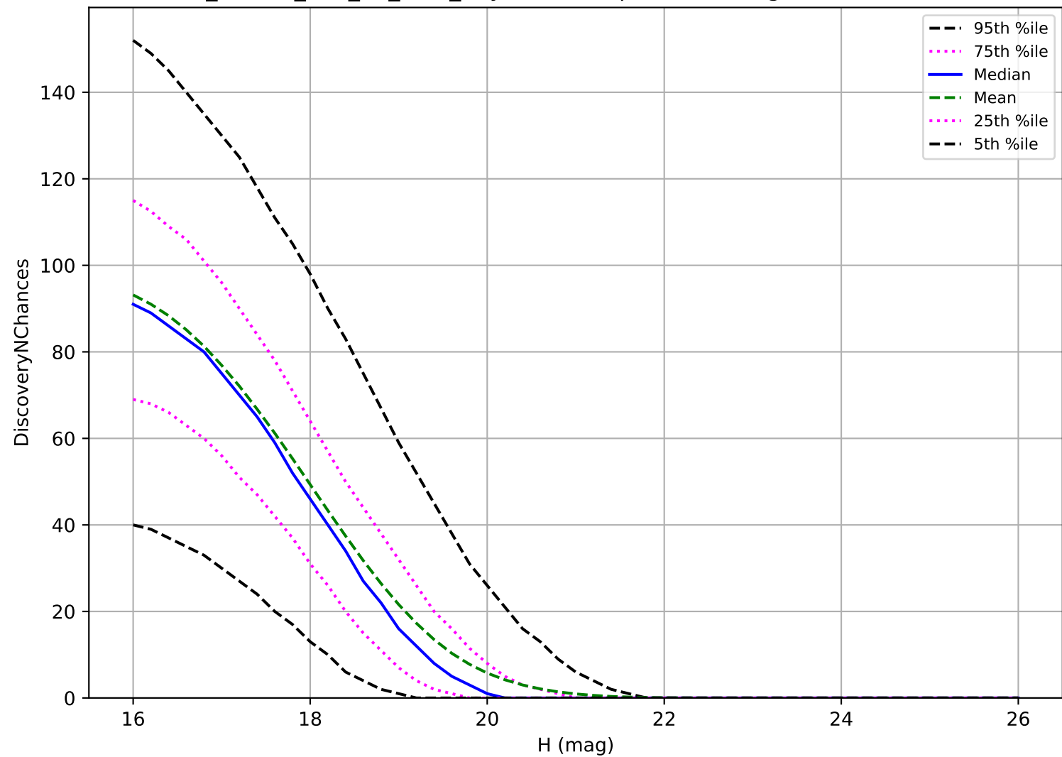
ddf_loaded_half_fl8_v3.4_10yrs: MBA 3 pairs in 15 nights detection loss
