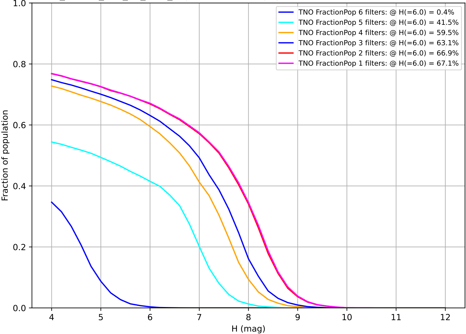
ddf_loaded_half_fl8_v3.4_10yrs: Fraction of population with colors in X filters TNO
