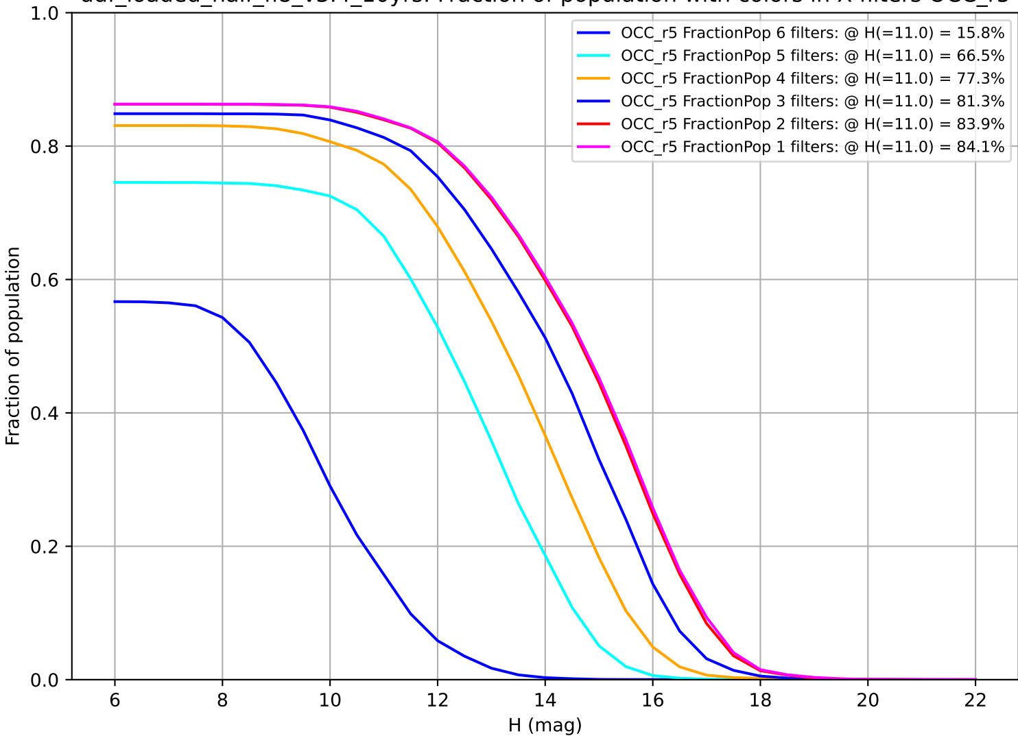
ddf_loaded_half_fl8_v3.4_10yrs: Fraction of population with colors in X filters OCC_r5
