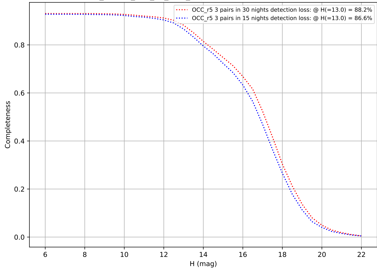
ddf_loaded_half_fl8_v3.4_10yrs: DifferentialCompleteness
