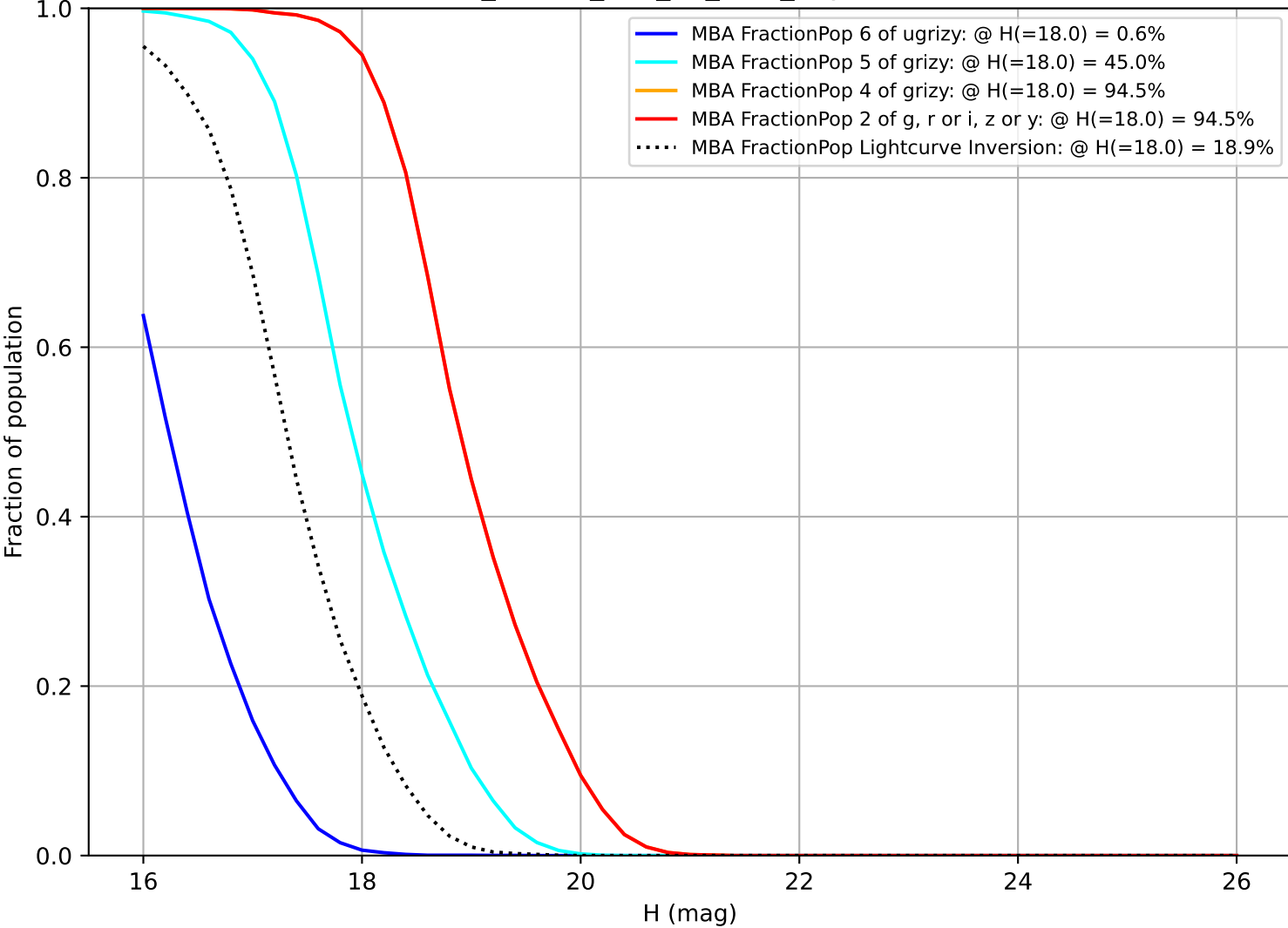
ddf_loaded_half_fl8_v3.4_10yrs MBA
