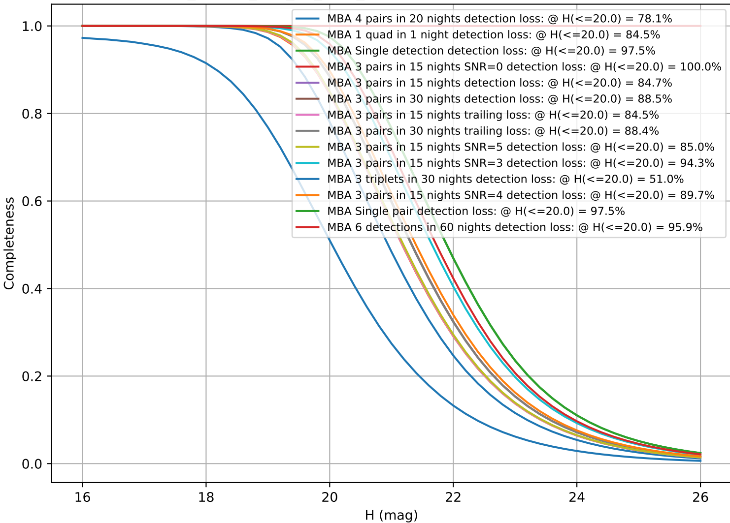
ddf_loaded_half_fl8_v3.4_10yrs: CumulativeCompleteness
