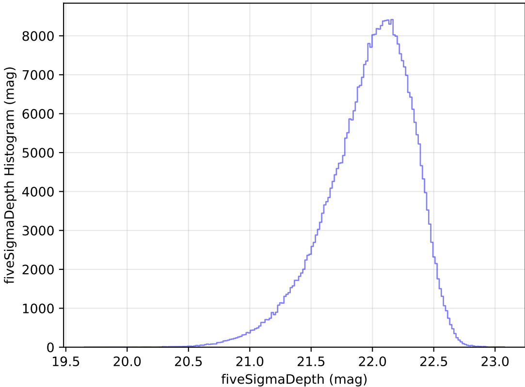
ddf_loaded_half_f18_v3.4_10yrs y: fiveSigmaDepth Histogram
