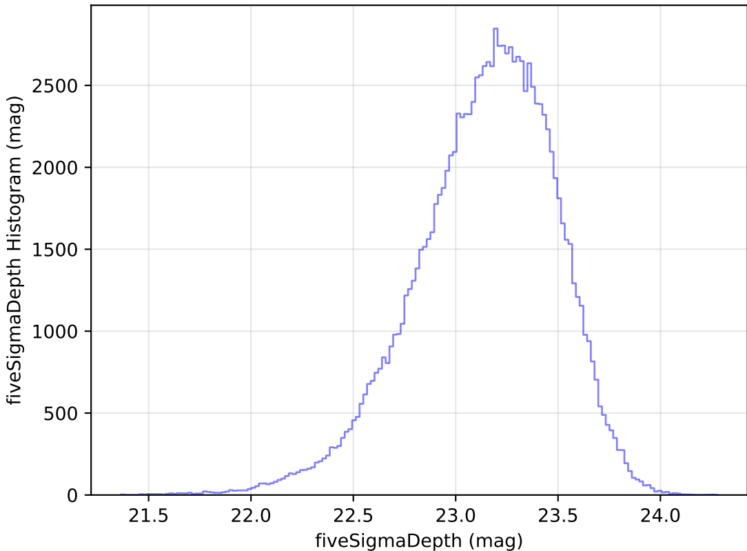
ddf_loaded_half_fl8_v3.4_10yrs u: fiveSigmaDepth Histogram
