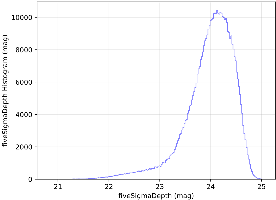
ddf_loaded_half_fl8_v3.4_10yrs r: fiveSigmaDepth Histogram
