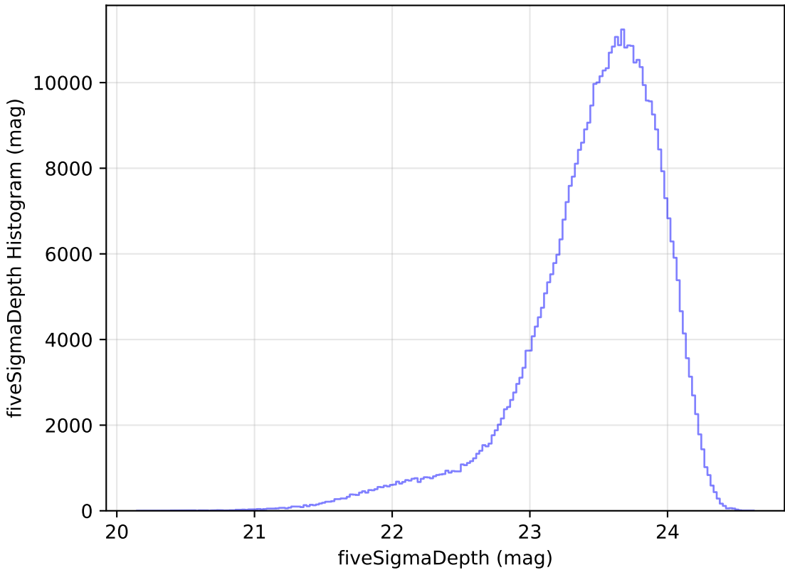
ddf_loaded_half_fl8_v3.4_10yrs i: fiveSigmaDepth Histogram
