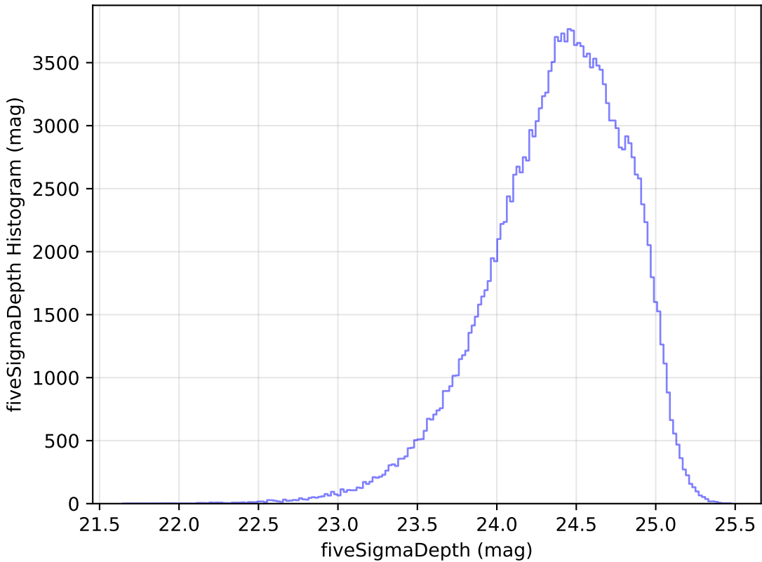
ddf_loaded_half_fl8_v3.4_10yrs g: fiveSigmaDepth Histogram
