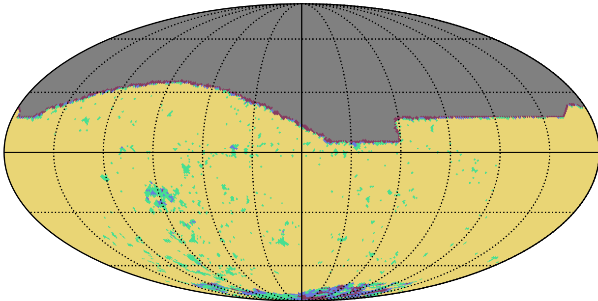
ddf_loaded_half_fl8_v3.4_10yrs i band: YearCoverage night
