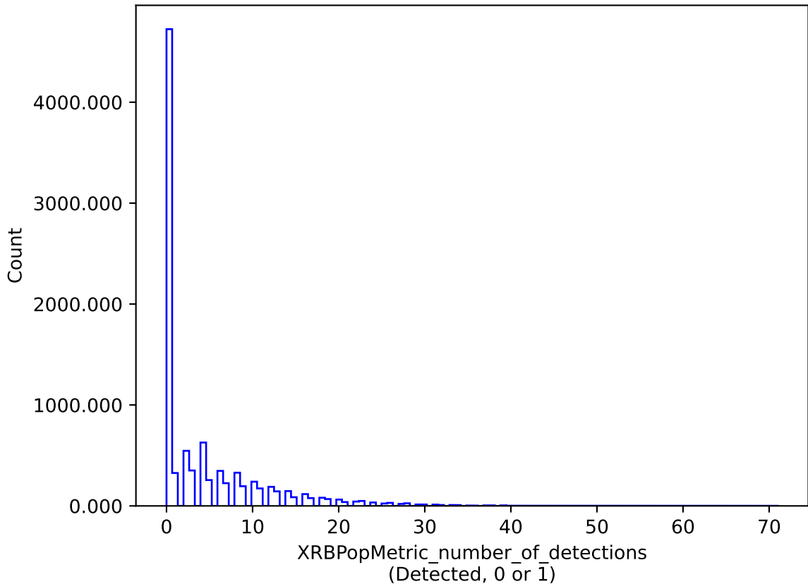
ddf_loaded_half_fl8_v3.4_10yrs : XRBPopMetric_number_of_detections
