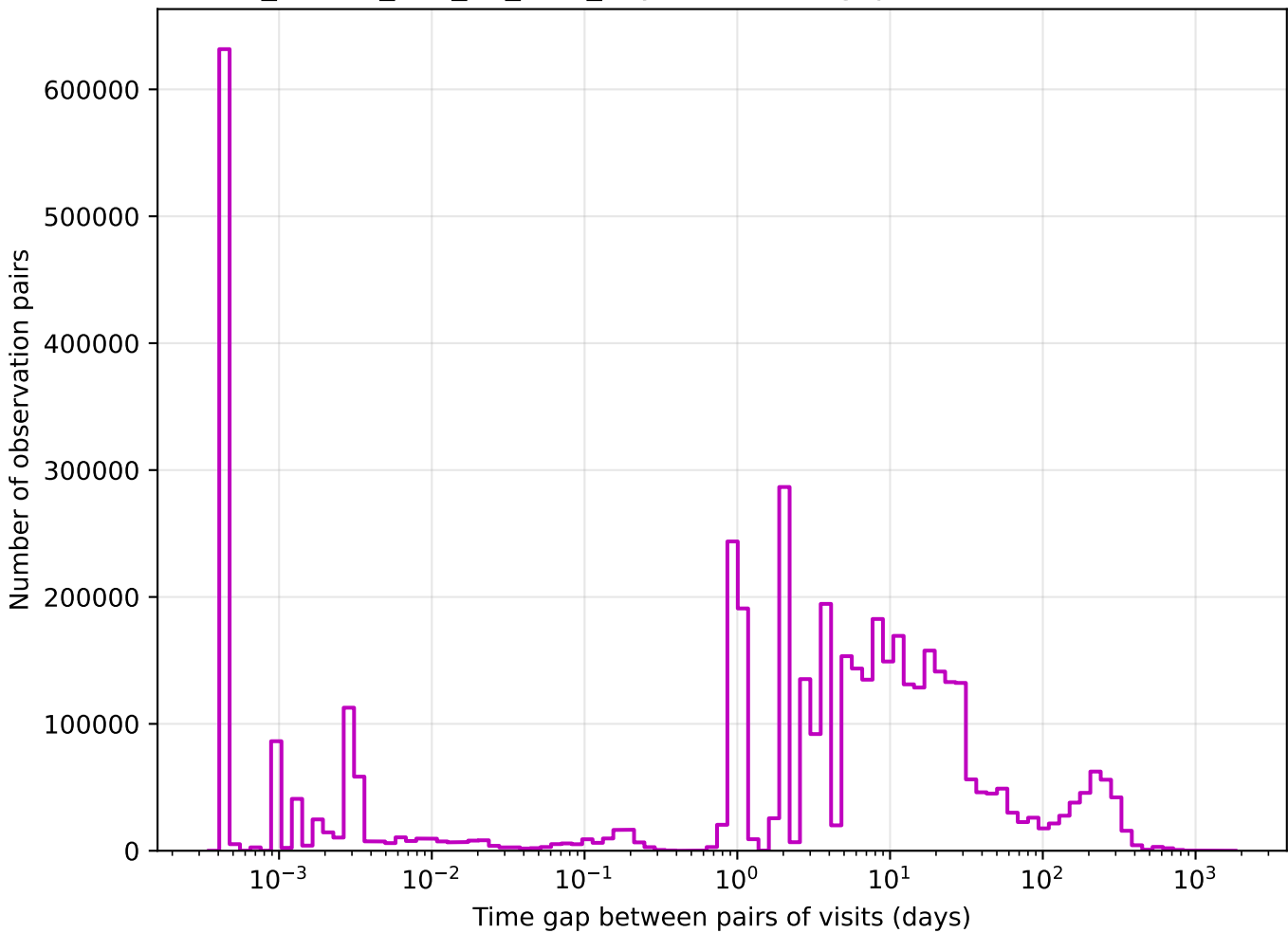
ddf_loaded_half_fl8_v3.4_10yrs z band: Tgaps observationStartMJD
