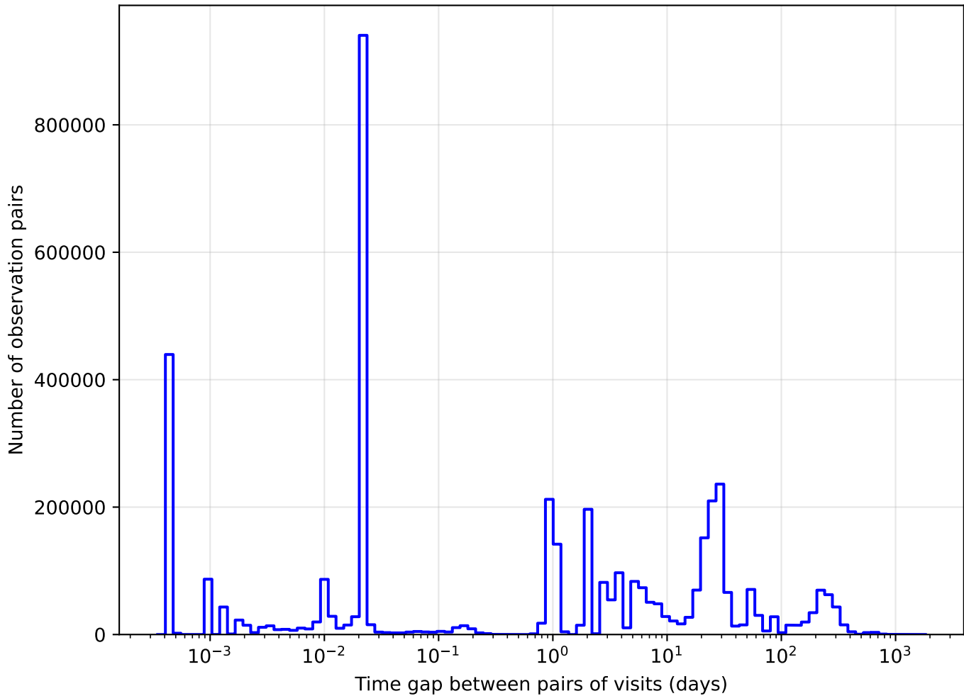
ddf_loaded_half_fl8_v3.4_10yrs y band: Tgaps observationStartMJD
