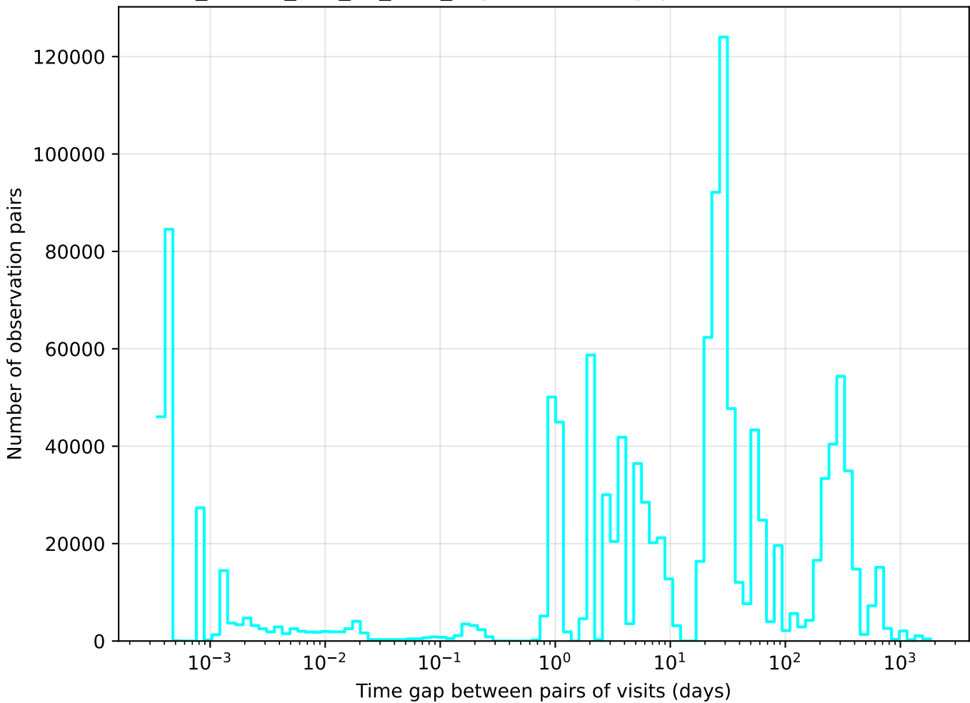
ddf_loaded_half_fl8_v3.4_10yrs u band: Tgaps observationStartMJD
