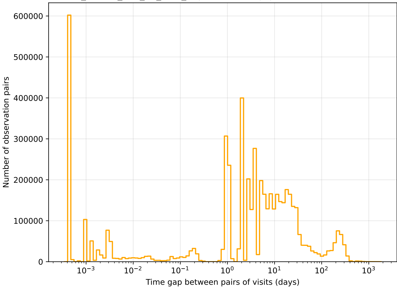
ddf_loaded_half_fl8_v3.4_10yrs r band: Tgaps observationStartMJD
