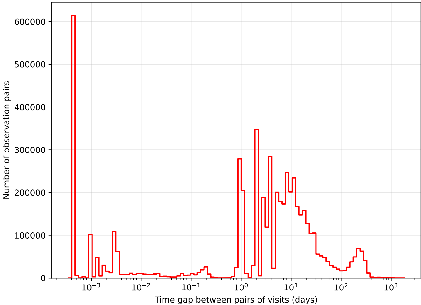
ddf_loaded_half_fi8_v3.4_10yrs i band: Tgaps observationStartMJD
