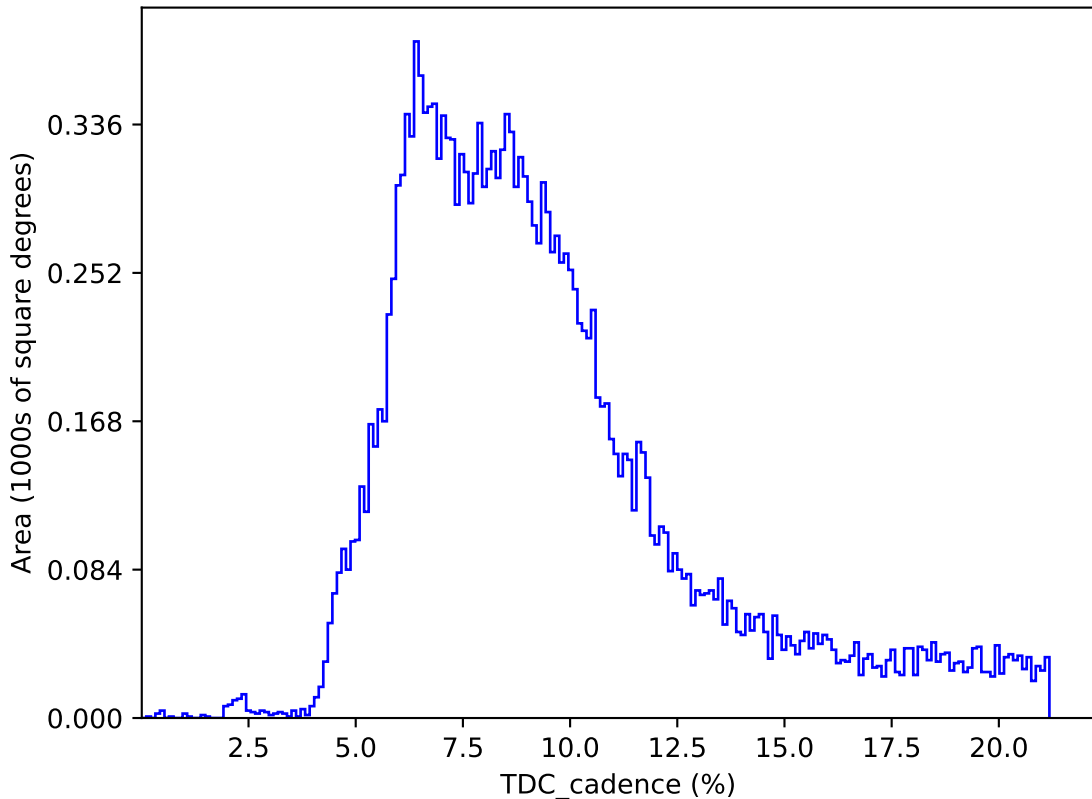
ddf_loaded_half_fl8_v3.4_10yrs : TDC_cadence
