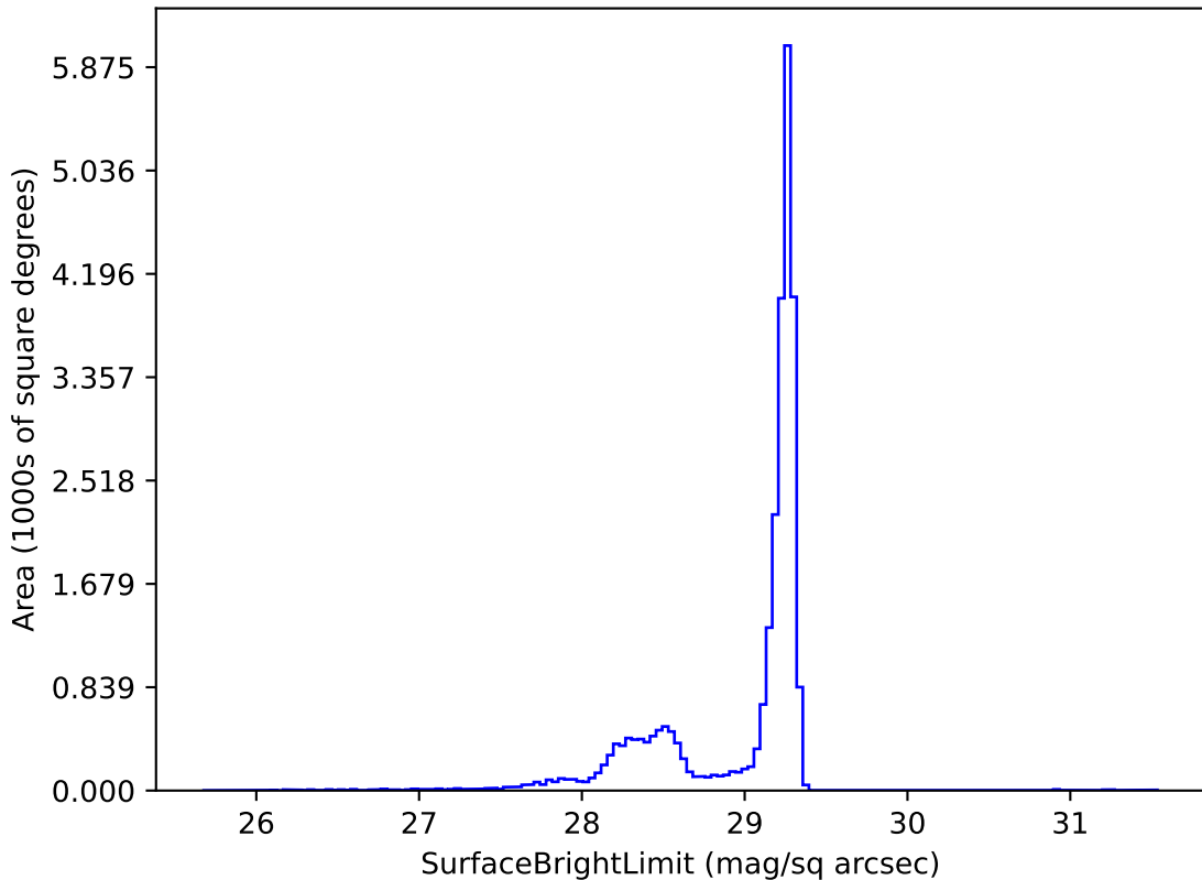
ddf_loaded_half_fl8_v3.4_10yrs z: SurfaceBrightLimit
