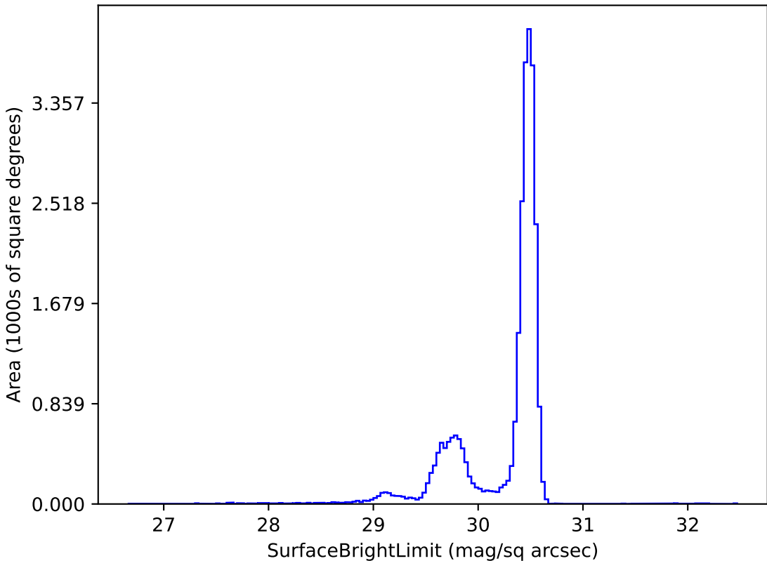
ddf_loaded_half_fl8_v3.4_10yrs r: SurfaceBrightLimit
