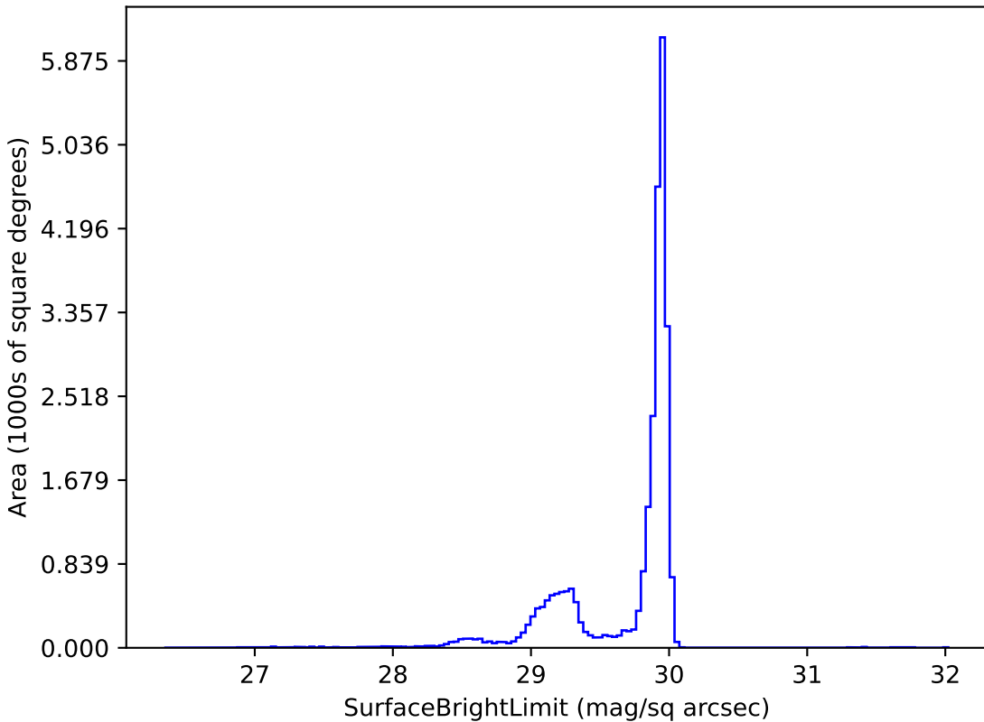
ddf_loaded_half_fl8_v3.4_10yrs i: SurfaceBrightLimit
